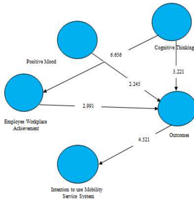
Figure 2. PLS Bootstrapping
